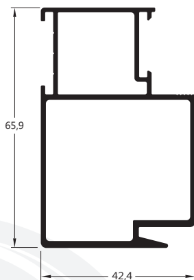
MG25-048 1,037 Kg/m Montante bi-tubular central interno
