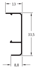
RA-613 0,162 Kg/m Remate
