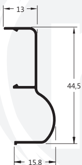
RA-1009 0,209 Kg/m Remate
