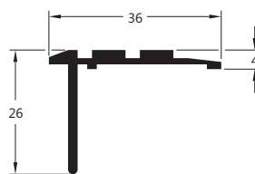
RA-516 0,339 Kg/m Remate
